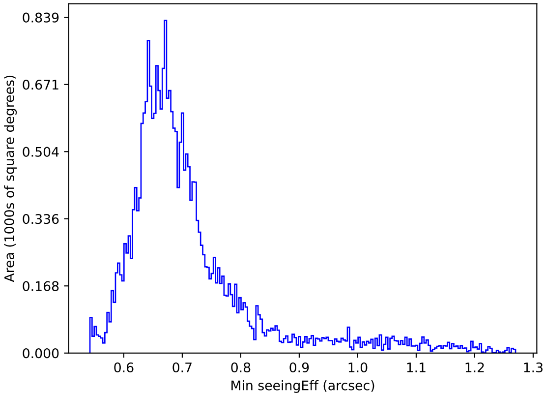
internal_u_expt27_nscale1.2v3.4_10yrs Yr 1 i band: Min seeingEff
