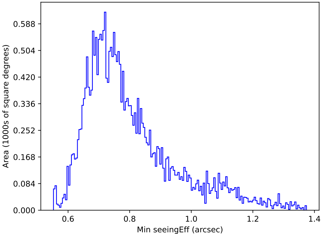
internal_u_expt27_nscale1.2v3.4_10yrs Yr 1 g band: Min seeingEff
