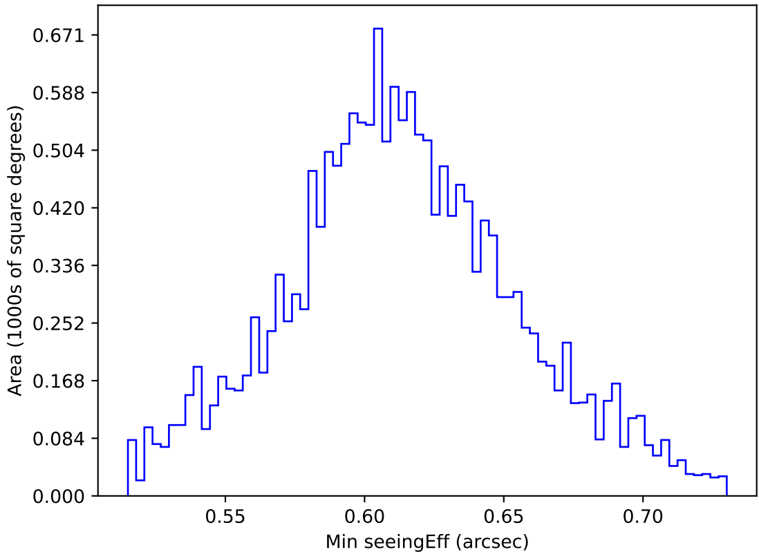
internal_u_expt27_nscale1.2v3.4_10yrs WFD z band: Min seeingEff
