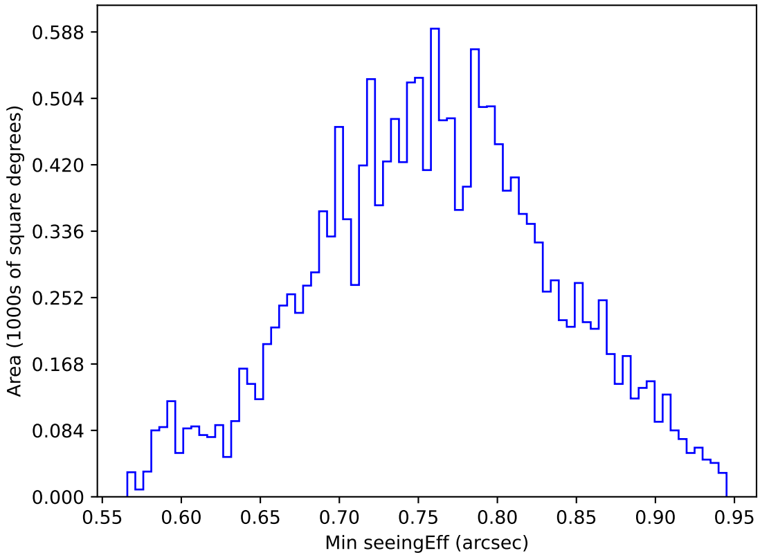
internal_u_expt27_nscale1.2v3.4_10yrs WFD u band: Min seeingEff
