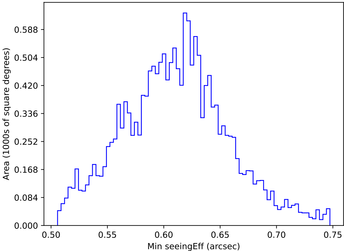
internal_u_expt27_nscale1.2v3.4_10yrs WFD r band: Min seeingEff
