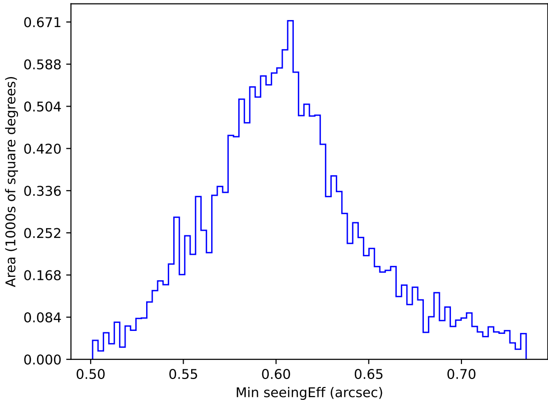
internal_u_expt27_nscale1.2v3.4_10yrs WFD i band: Min seeingEff
