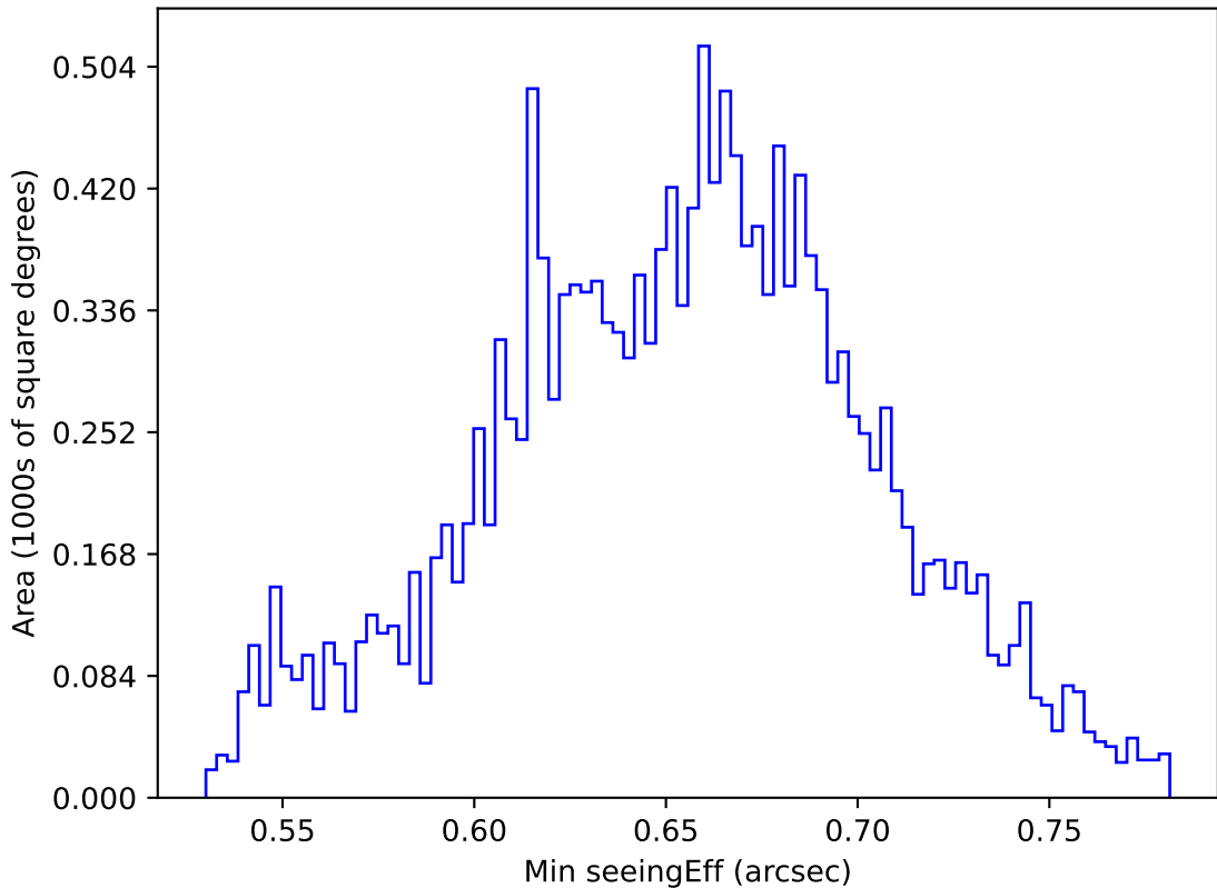
internal_u_expt27_nscale1.2v3.4_10yrs WFD g band: Min seeingEff
