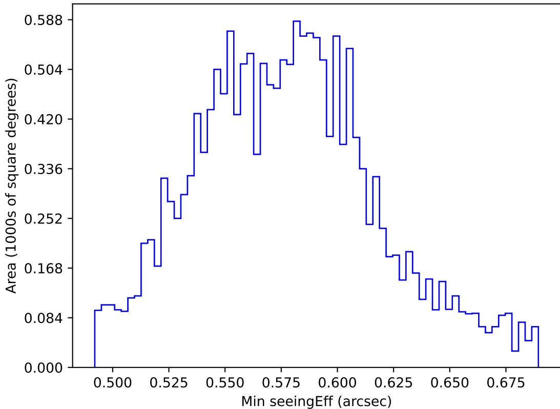
internal_u_expt27_nscale1.2v3.4_10yrs WFD all bands: Min seeingEff
