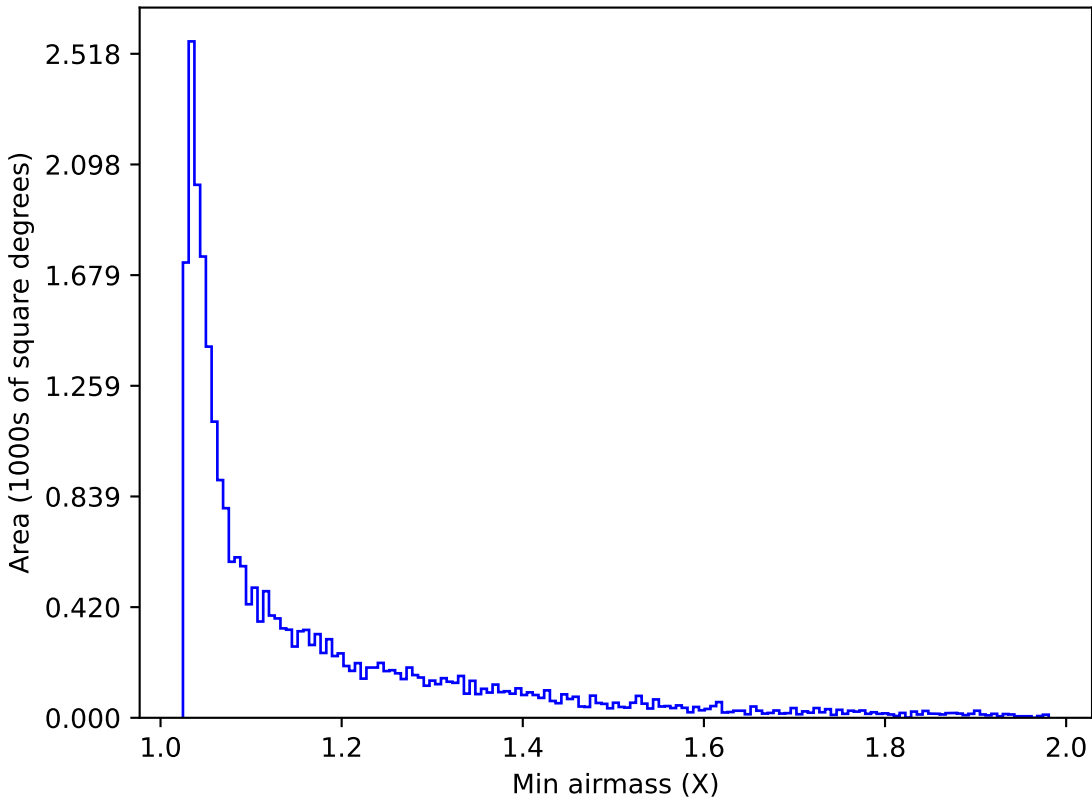
internal_u_expt27_nscale1.2v3.4_10yrs Yr 1 z band: Min airmass
