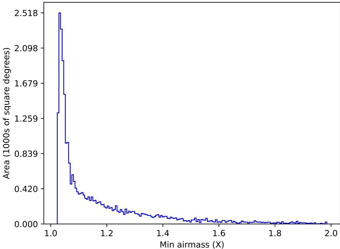
internal_u_expt27_nscale1.2v3.4_10yrs Yr 1 i band: Min airmass
