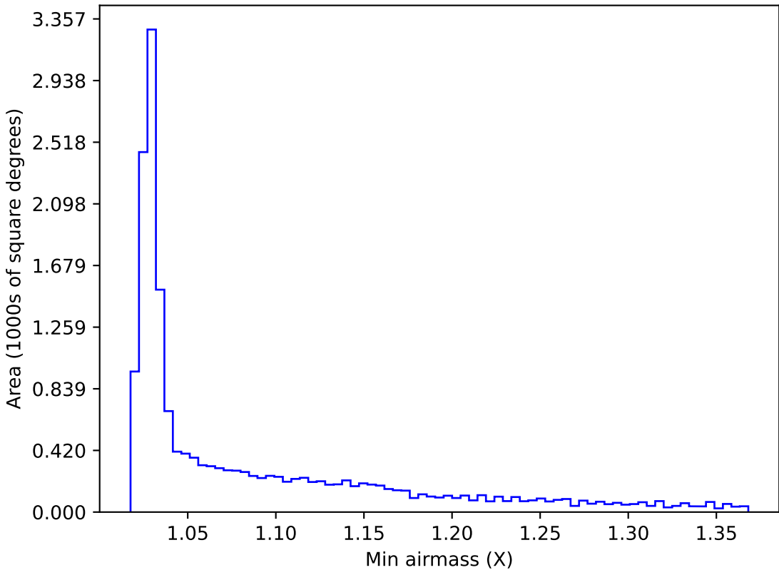
internal_u_expt27_nscale1.2v3.4_10yrs WFD i band: Min airmass
