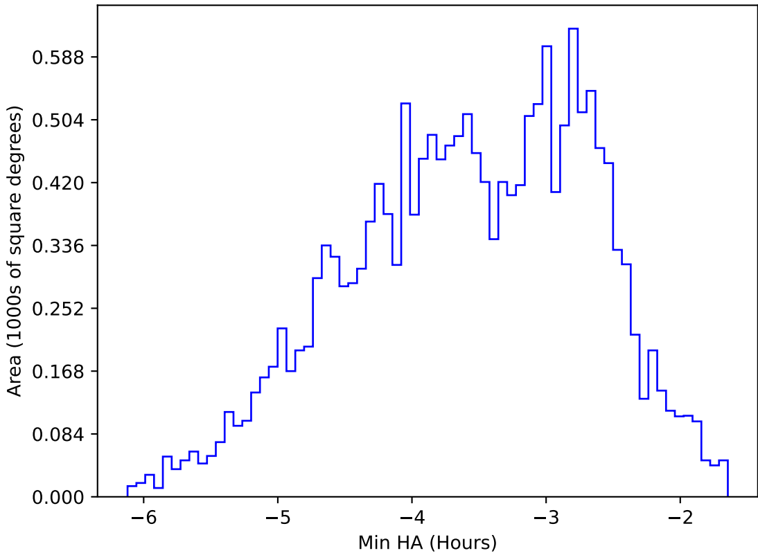
internal_u_expt27_nscale1.2v3.4_10yrs WFD y band: Min HA
