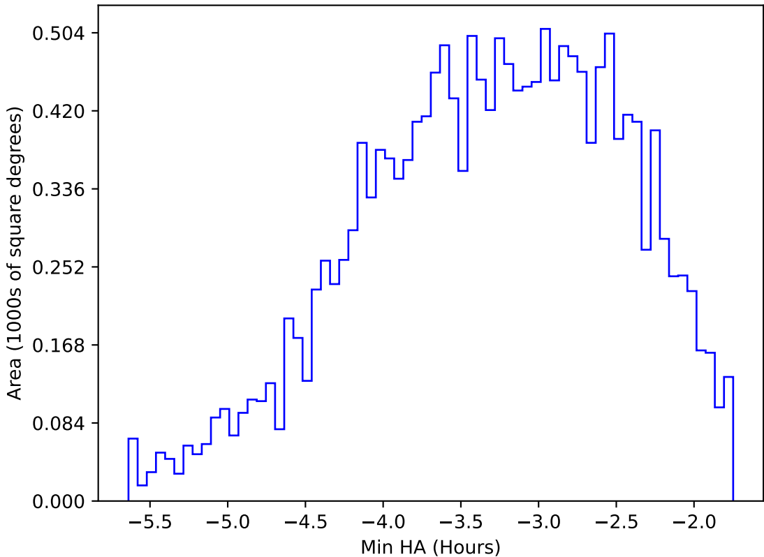
internal_u_expt27_nscale1.2v3.4_10yrs WFD u band: Min HA
