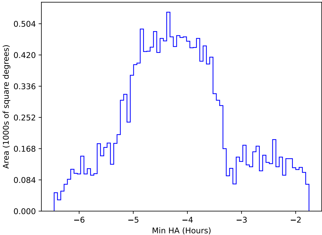
internal_u_expt27_nscale1.2v3.4_10yrs WFD g band: Min HA
