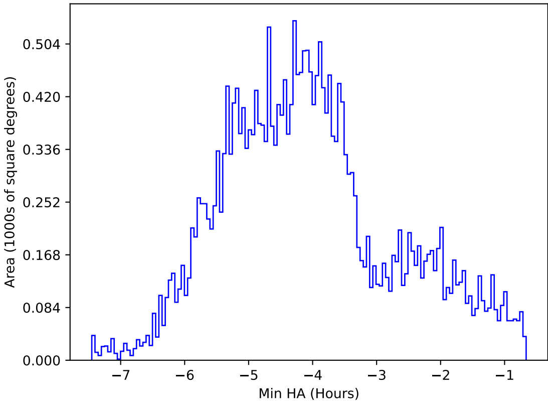
internal_u_expt27_nscale1.2v3.4_10yrs All sky z band: Min HA
