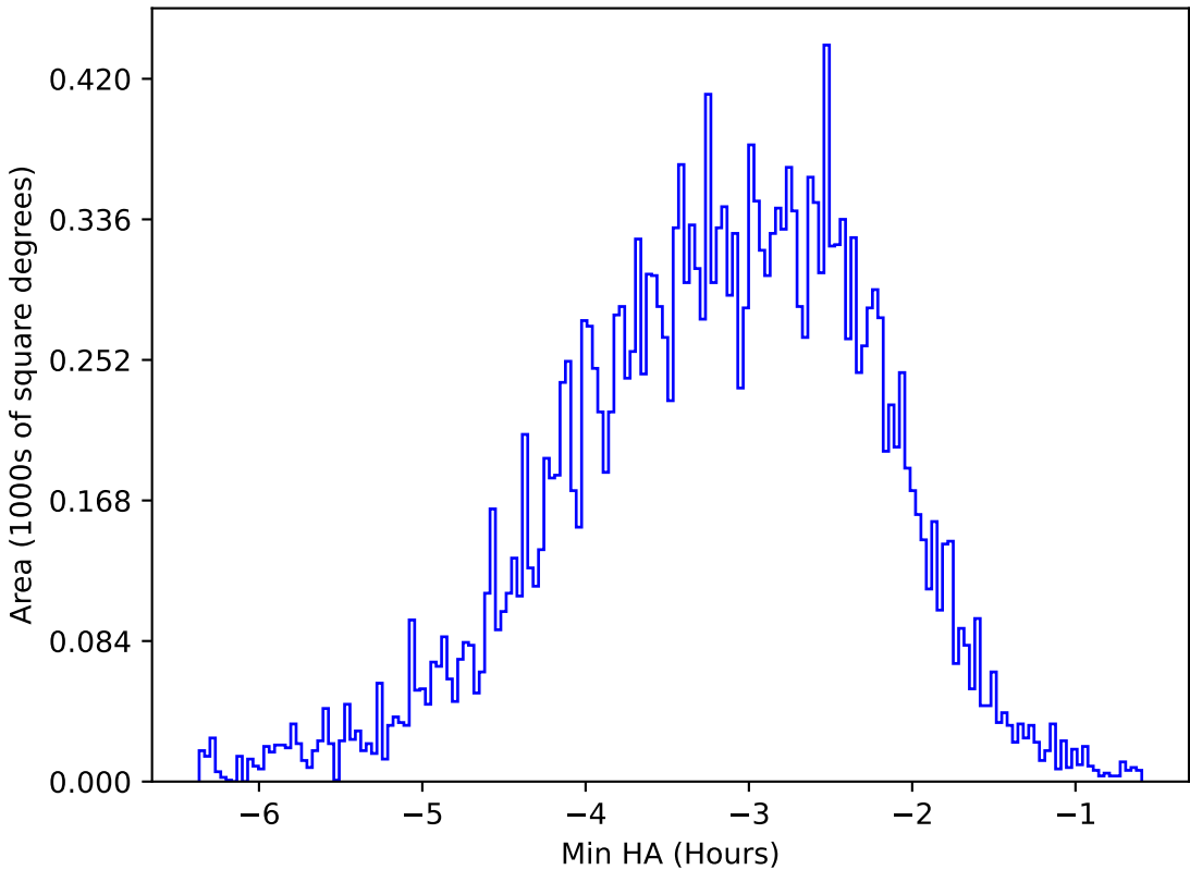
internal_u_expt27_nscale1.2v3.4_10yrs All sky u band: Min HA
