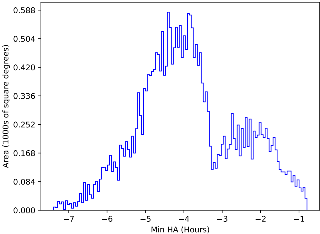
internal_u_expt27_nscale1.2v3.4_10yrs All sky g band: Min HA
