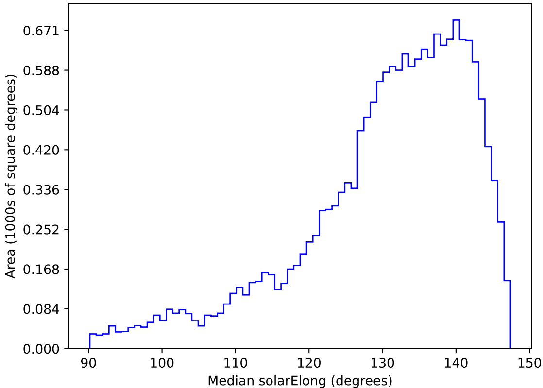
internal_u_expt27_nscale1.2v3.4_10yrs WFD r band: Median solarElong
