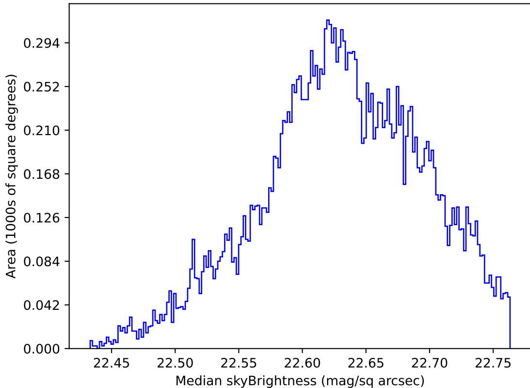
internal_u_expt27_nscale1.2v3.4_10yrs Yr 1 u band: Median skyBrightness
