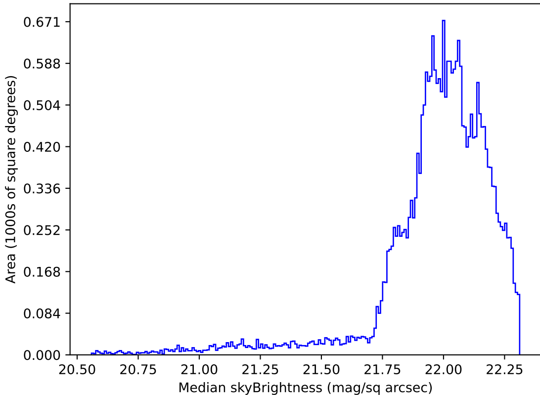
internal_u_expt27_nscale1.2v3.4_10yrs Yr 1 g band: Median skyBrightness
