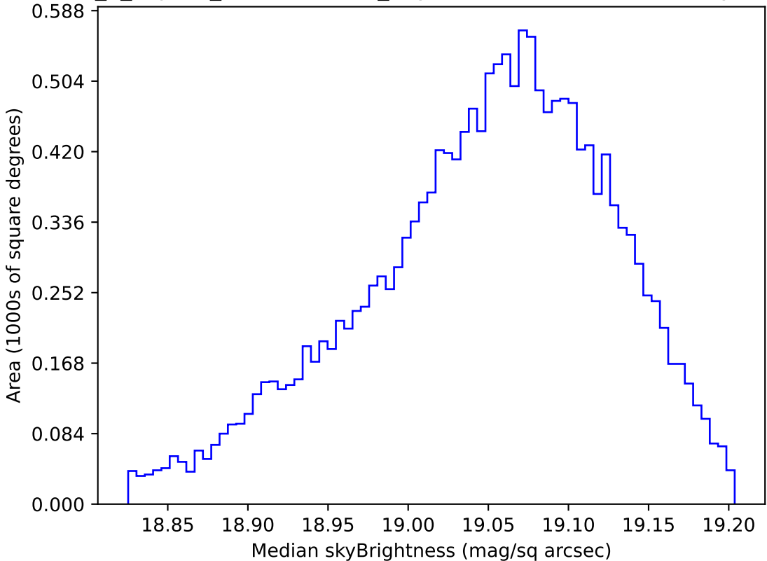
internal_u_expt27_nscale1.2v3.4_10yrs WFD z band: Median skyBrightness
