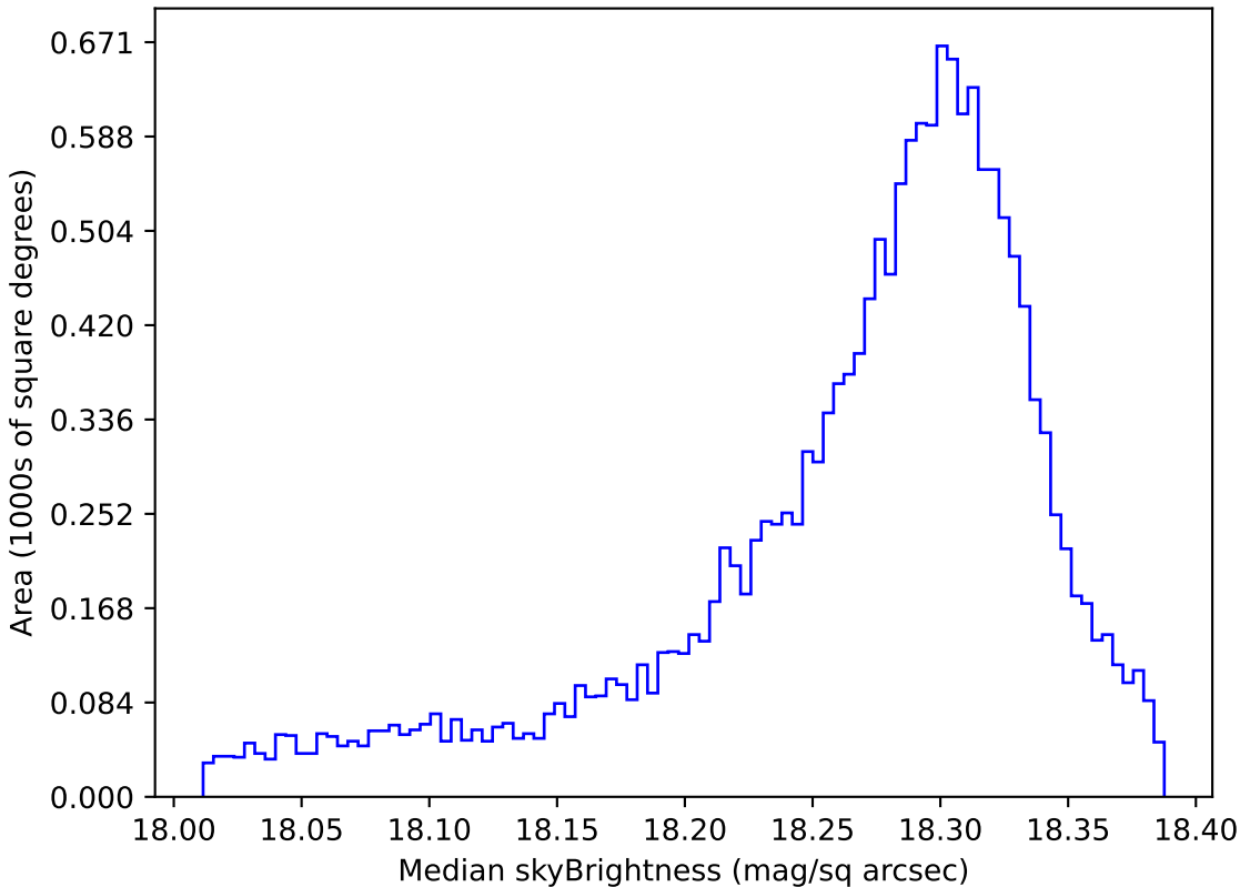
internal_u_expt27_nscale1.2v3.4_10yrs WFD y band: Median skyBrightness
