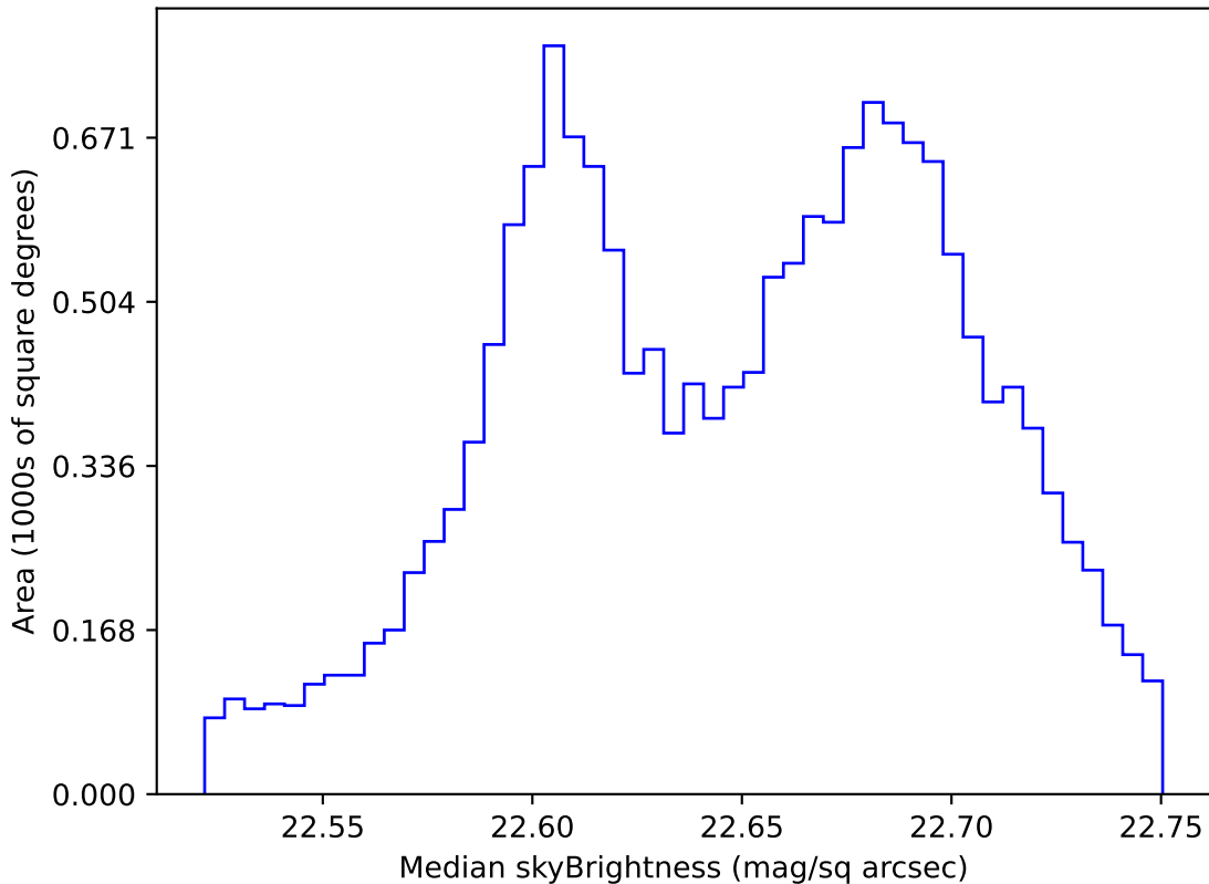
internal_u_expt27_nscale1.2v3.4_10yrs WFD u band: Median skyBrightness
