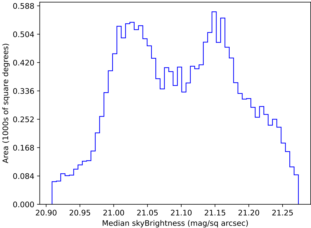
internal_u_expt27_nscale1.2v3.4_10yrs WFD r band: Median skyBrightness
