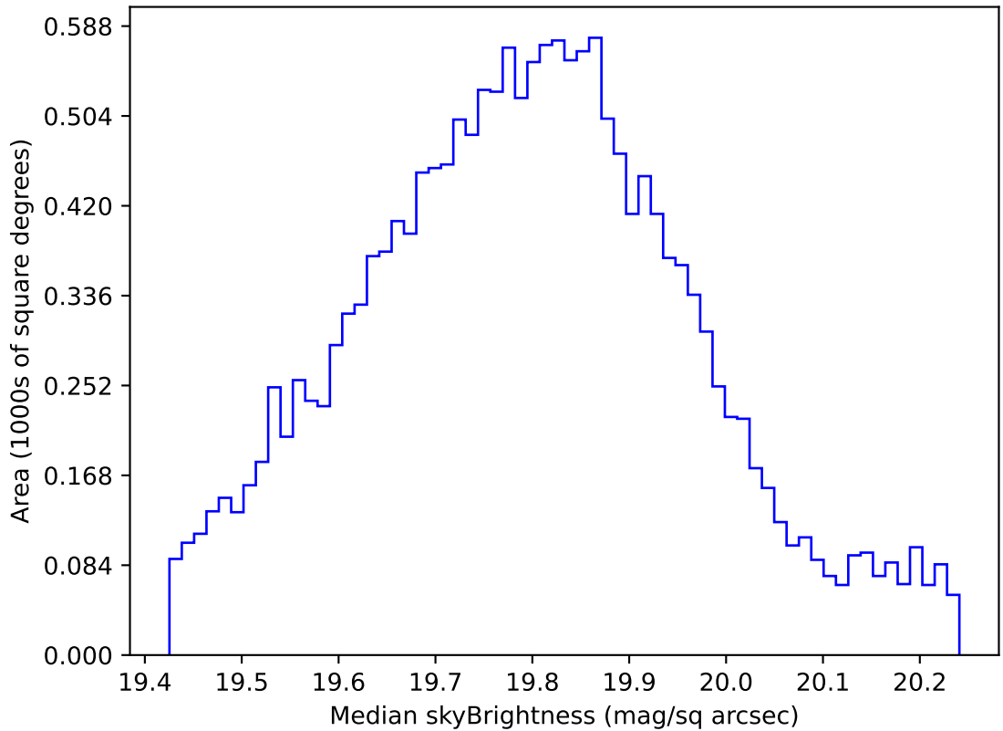
internal_u_expt27_nscale1.2v3.4_10yrs WFD all bands: Median skyBrightness
