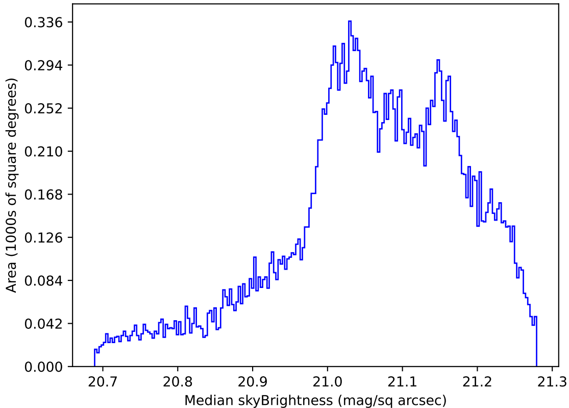
internal_u_expt27_nscale1.2v3.4_10yrs All sky r band: Median skyBrightness
