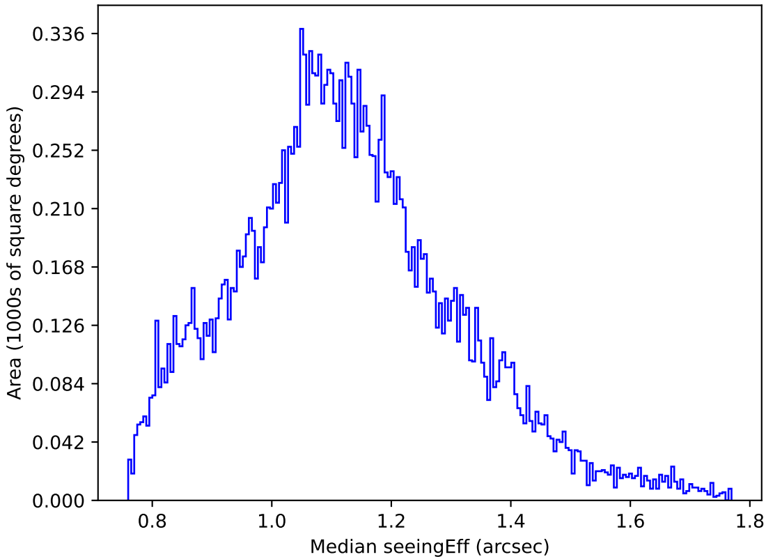
internal_u_expt27_nscale1.2v3.4_10yrs Yr 1 u band: Median seeingEff
