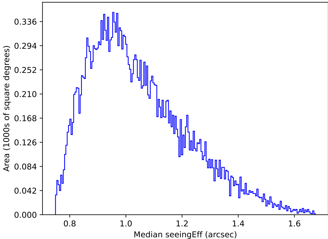
internal_u_expt27_nscale1.2v3.4_10yrs Yr 1 g band: Median seeingEff
