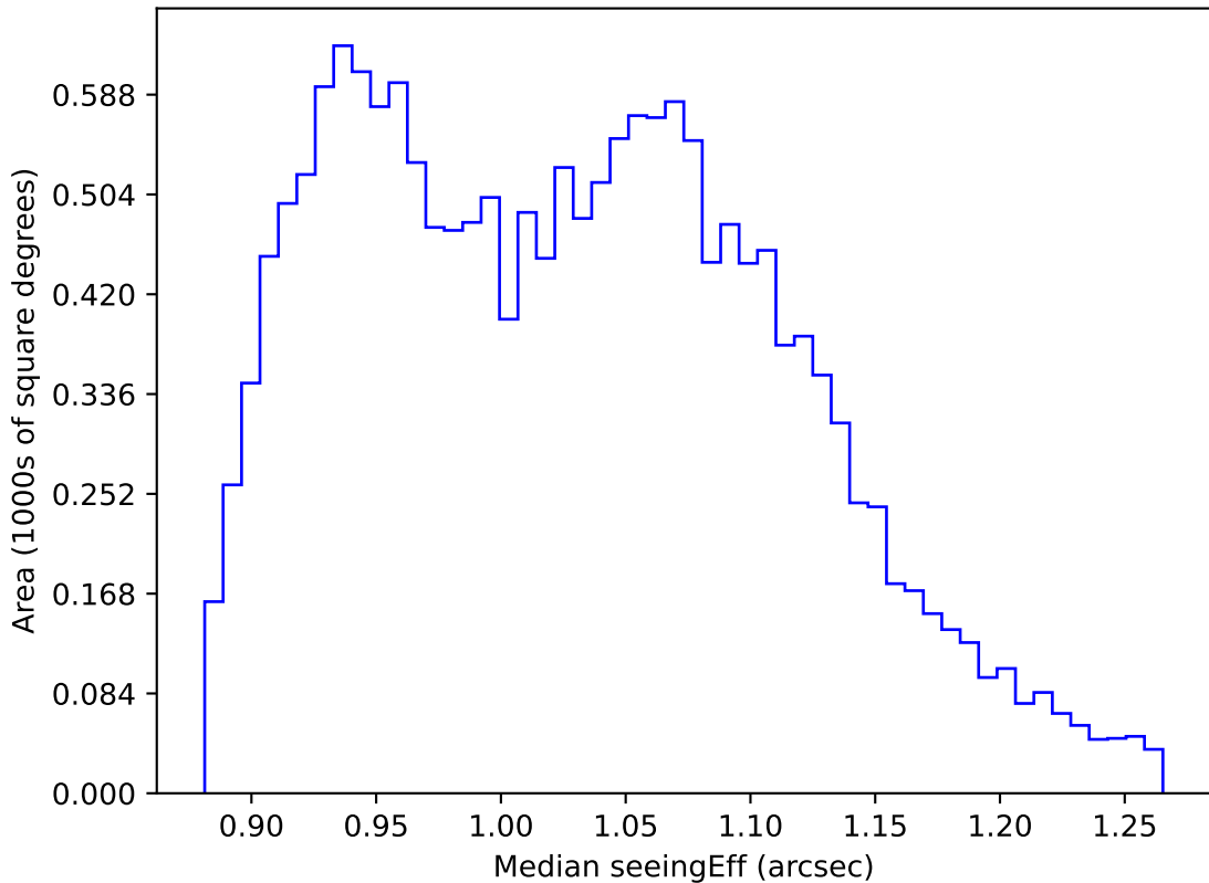
internal_u_expt27_nscale1.2v3.4_10yrs WFD r band: Median seeingEff
