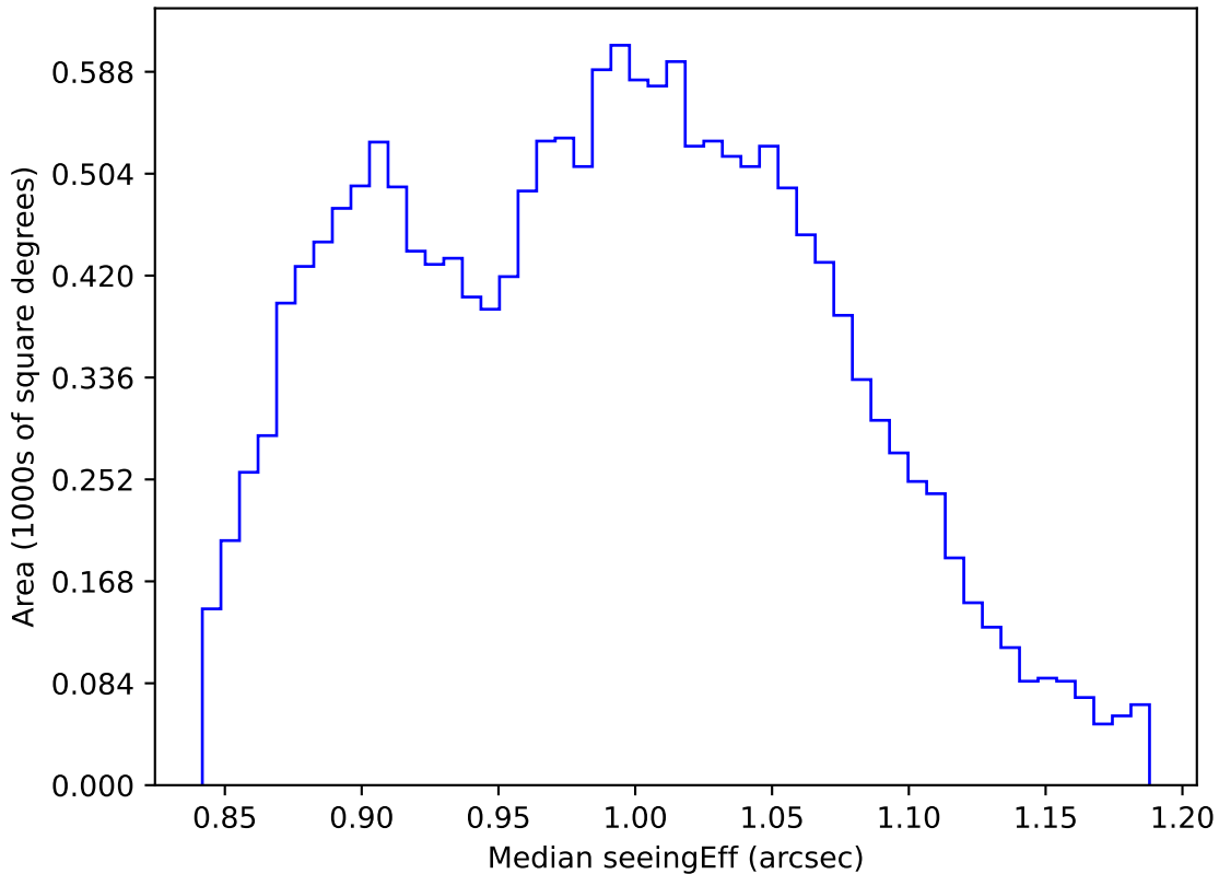
internal_u_expt27_nscale1.2v3.4_10yrs WFD i band: Median seeingEff
