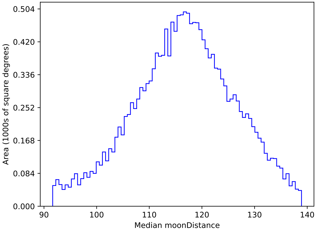
internal_u_expt27_nscale1.2v3.4_10yrs WFD g band: Median moonDistance
