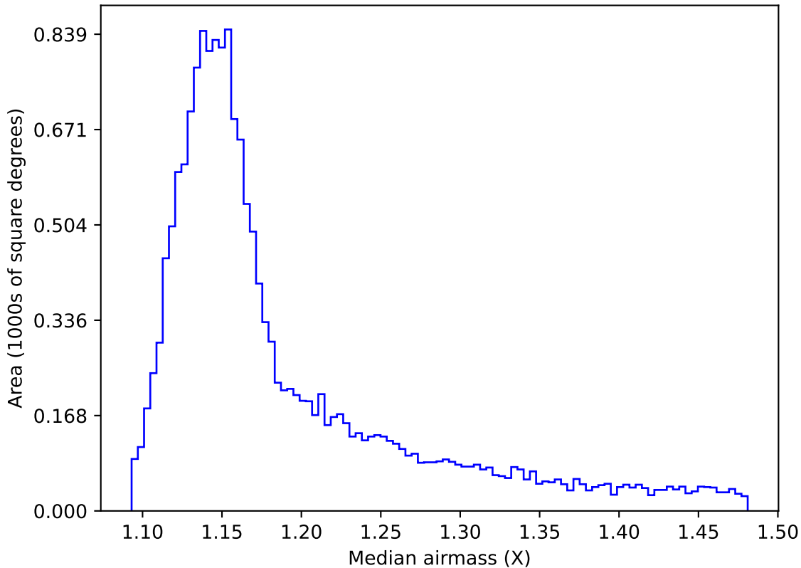
internal_u_expt27_nscale1.2v3.4_10yrs WFD y band: Median airmass
