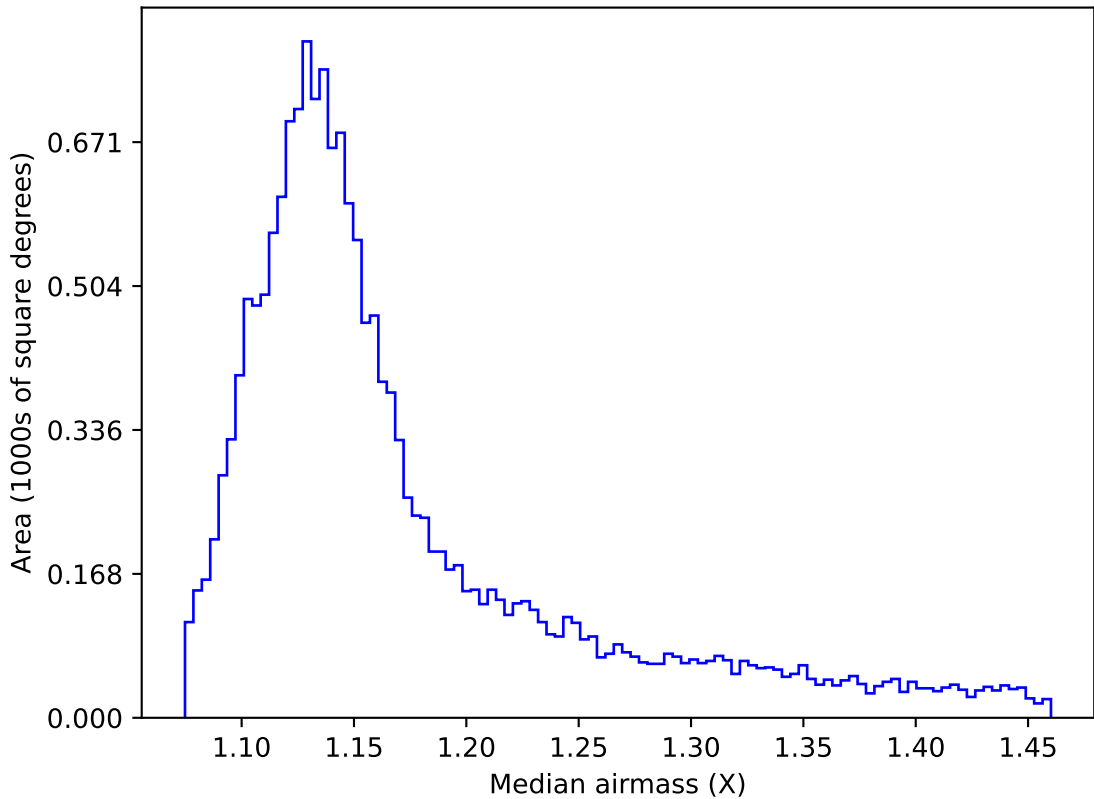
internal_u_expt27_nscale1.2v3.4_10yrs WFD r band: Median airmass
