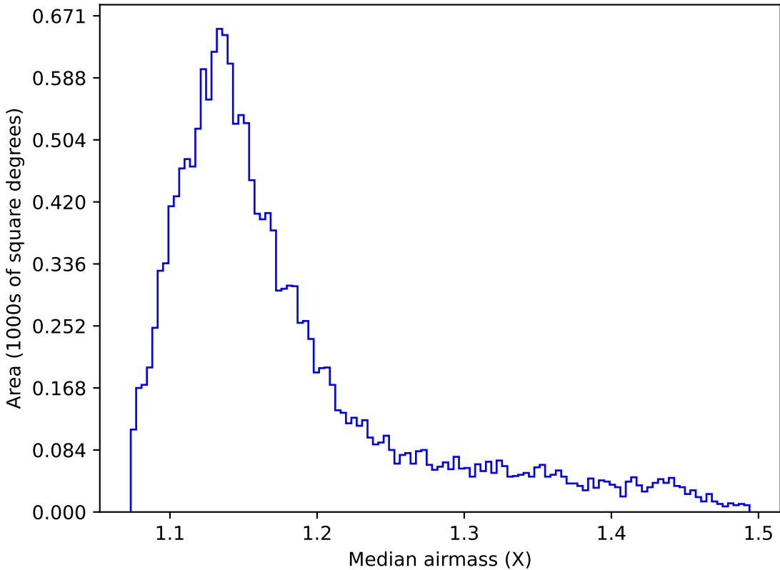
internal_u_expt27_nscale1.2v3.4_10yrs WFD g band: Median airmass
