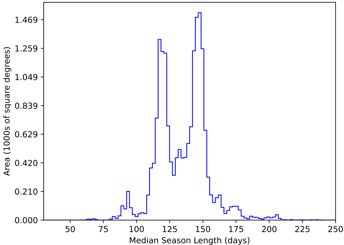
internal_u_expt27_nscale1.2v3.4_10yrs WFD y band: Median Season Length
