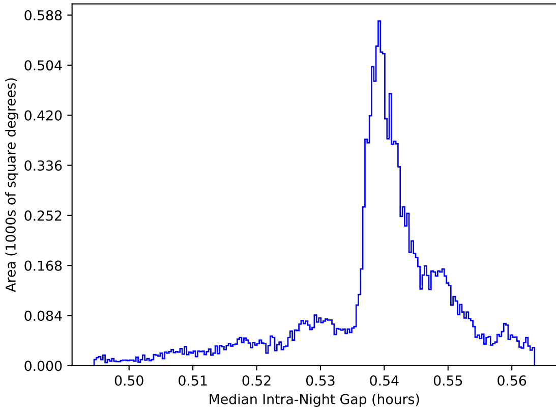
internal_u_expt27_nscale1.2v3.4_10yrs WFD: Median Intra-Night Gap
