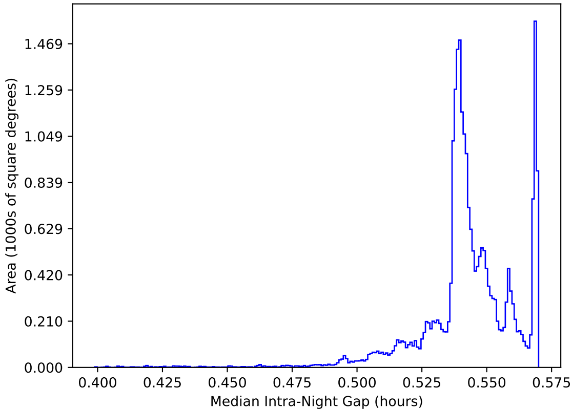
internal_u_expt27_nscale1.2v3.4_10yrs All sky: Median Intra-Night Gap
