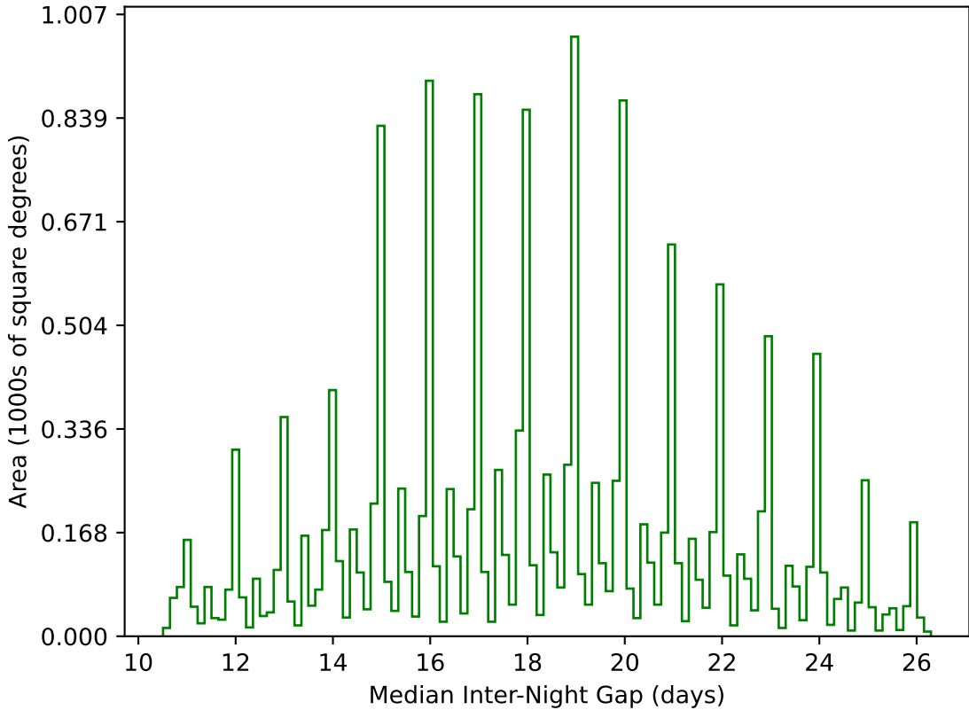
internal_u_expt27_nscale1.2v3.4_10yrs WFD g band: Median Inter-Night Gap
