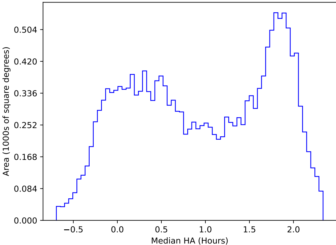
internal_u_expt27_nscale1.2v3.4_10yrs WFD u band: Median HA
