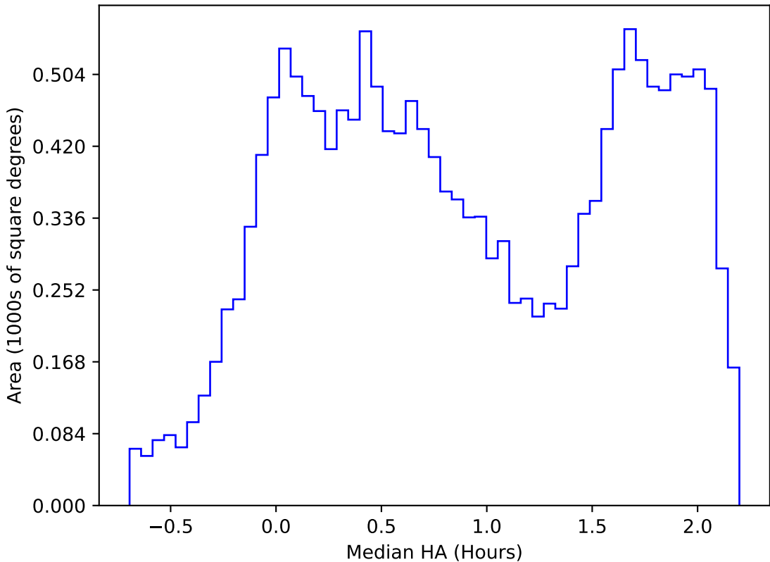
internal_u_expt27_nscale1.2v3.4_10yrs WFD r band: Median HA
