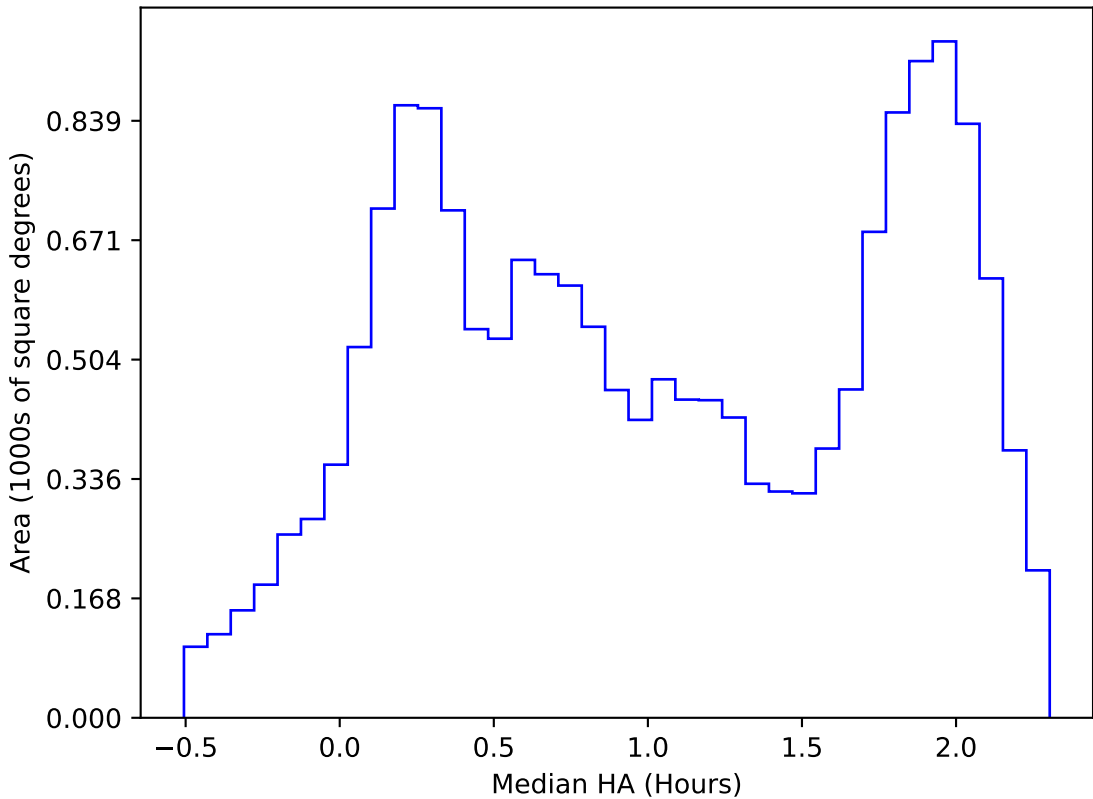
internal_u_expt27_nscale1.2v3.4_10yrs WFD i band: Median HA
