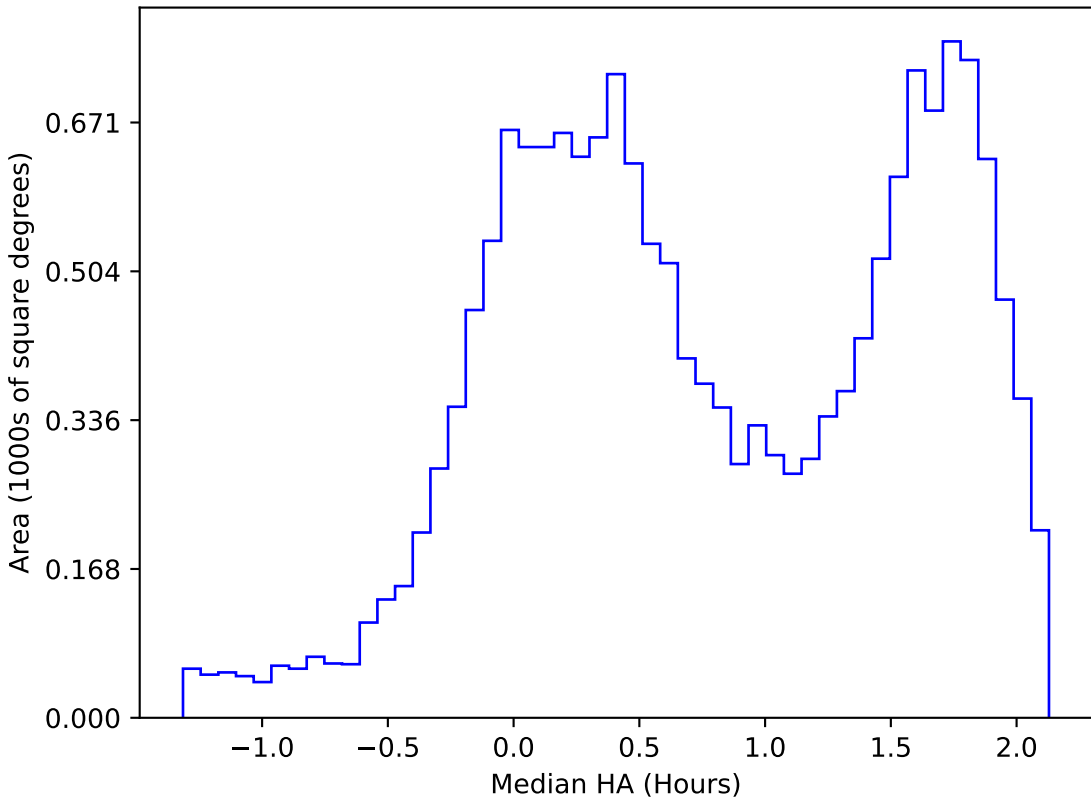
internal_u_expt27_nscale1.2v3.4_10yrs WFD g band: Median HA
