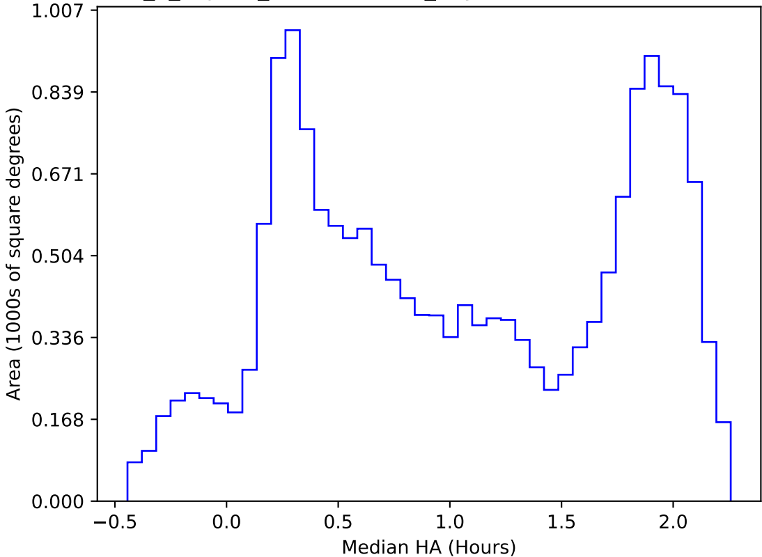
internal_u_expt27_nscale1.2v3.4_10yrs WFD all bands: Median HA
