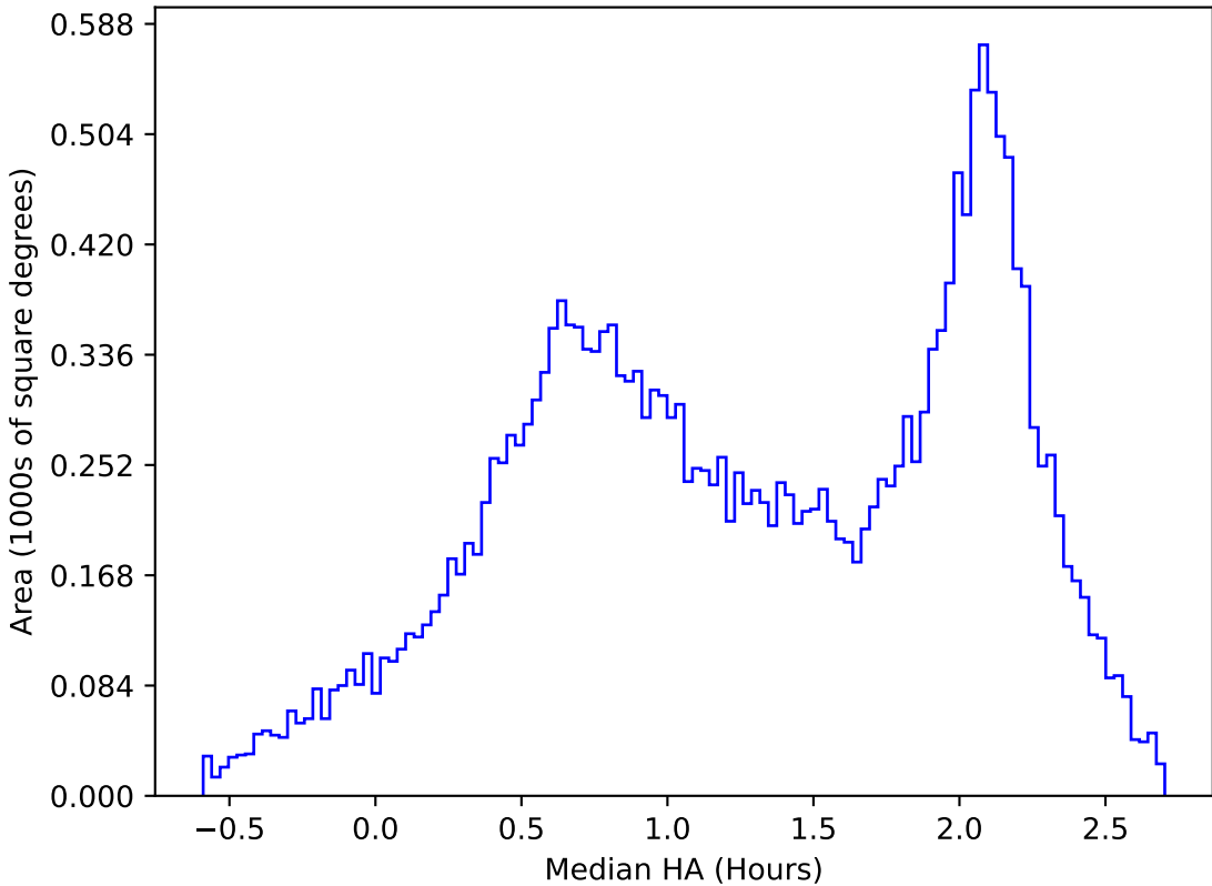
internal_u_expt27_nscale1.2v3.4_10yrs All sky y band: Median HA
