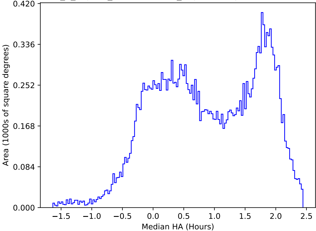
internal_u_expt27_nscale1.2v3.4_10yrs All sky u band: Median HA
