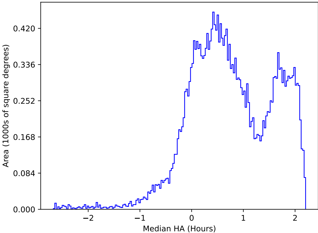
internal_u_expt27_nscale1.2v3.4_10yrs All sky r band: Median HA
