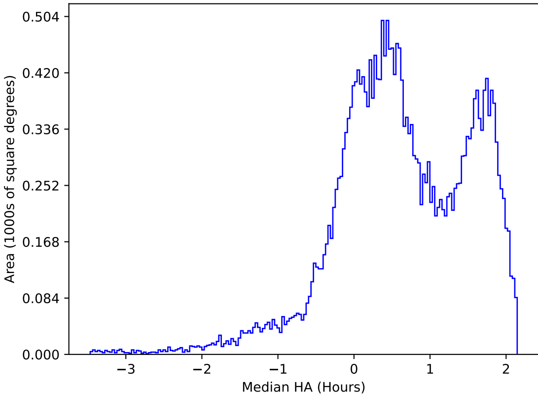
internal_u_expt27_nscale1.2v3.4_10yrs All sky g band: Median HA
