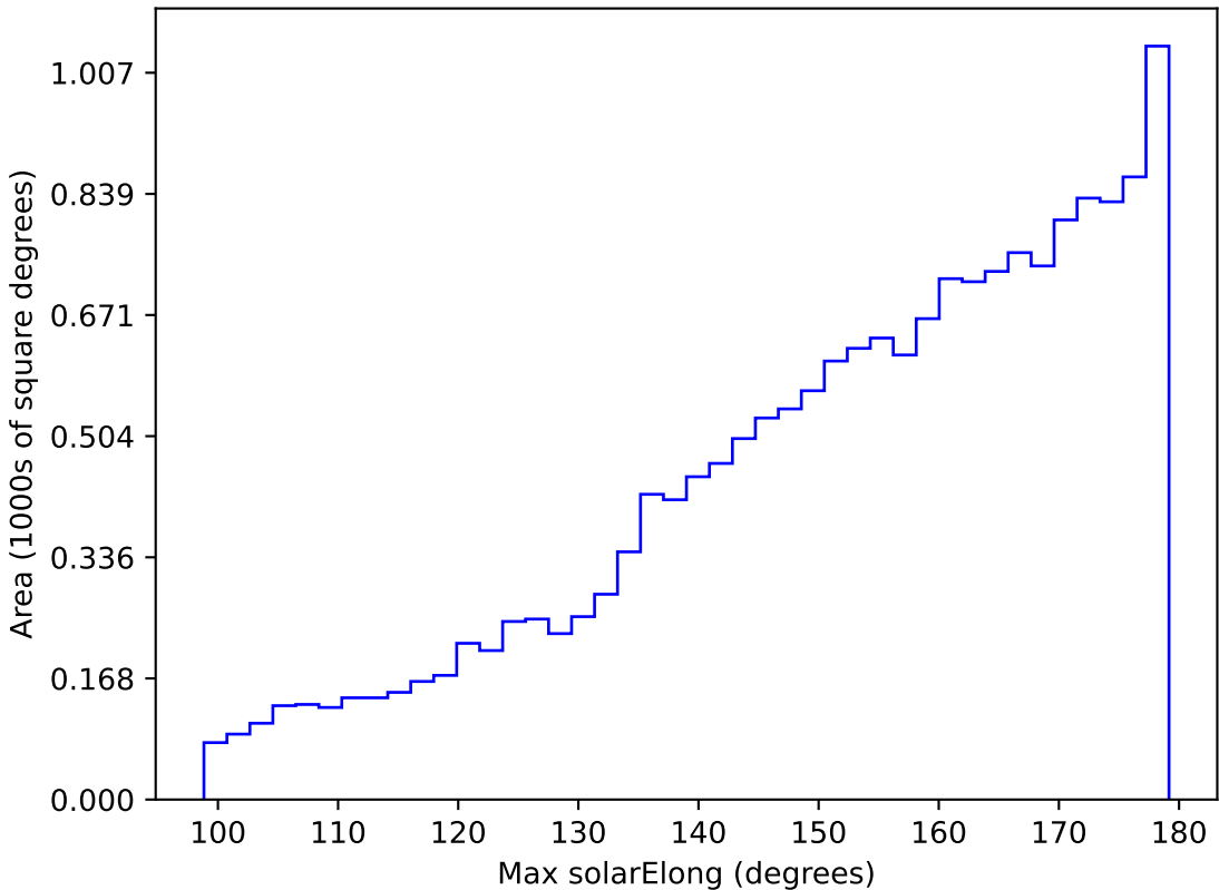
internal_u_expt27_nscale1.2v3.4_10yrs WFD y band: Max solarElong
