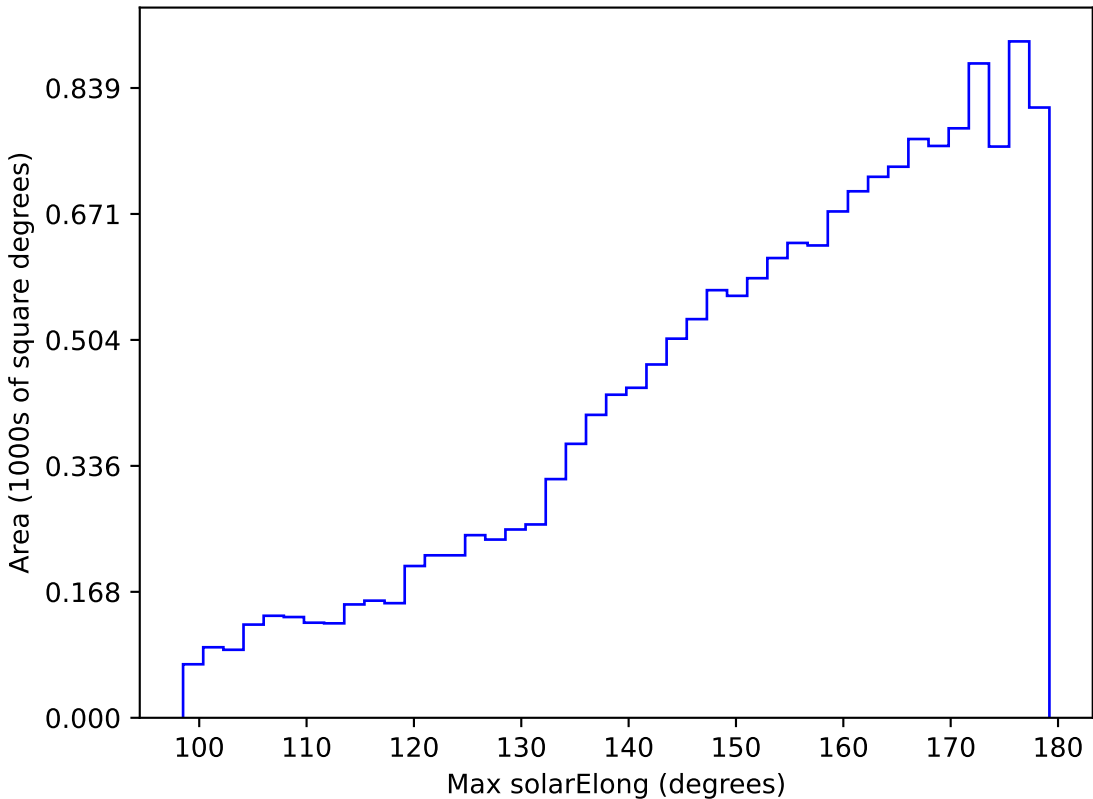
internal_u_expt27_nscale1.2v3.4_10yrs WFD g band: Max solarElong
