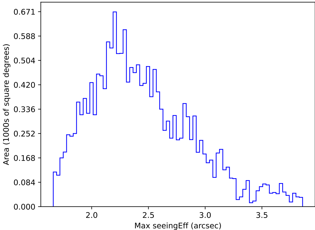
internal_u_expt27_nscale1.2v3.4_10yrs WFD g band: Max seeingEff
